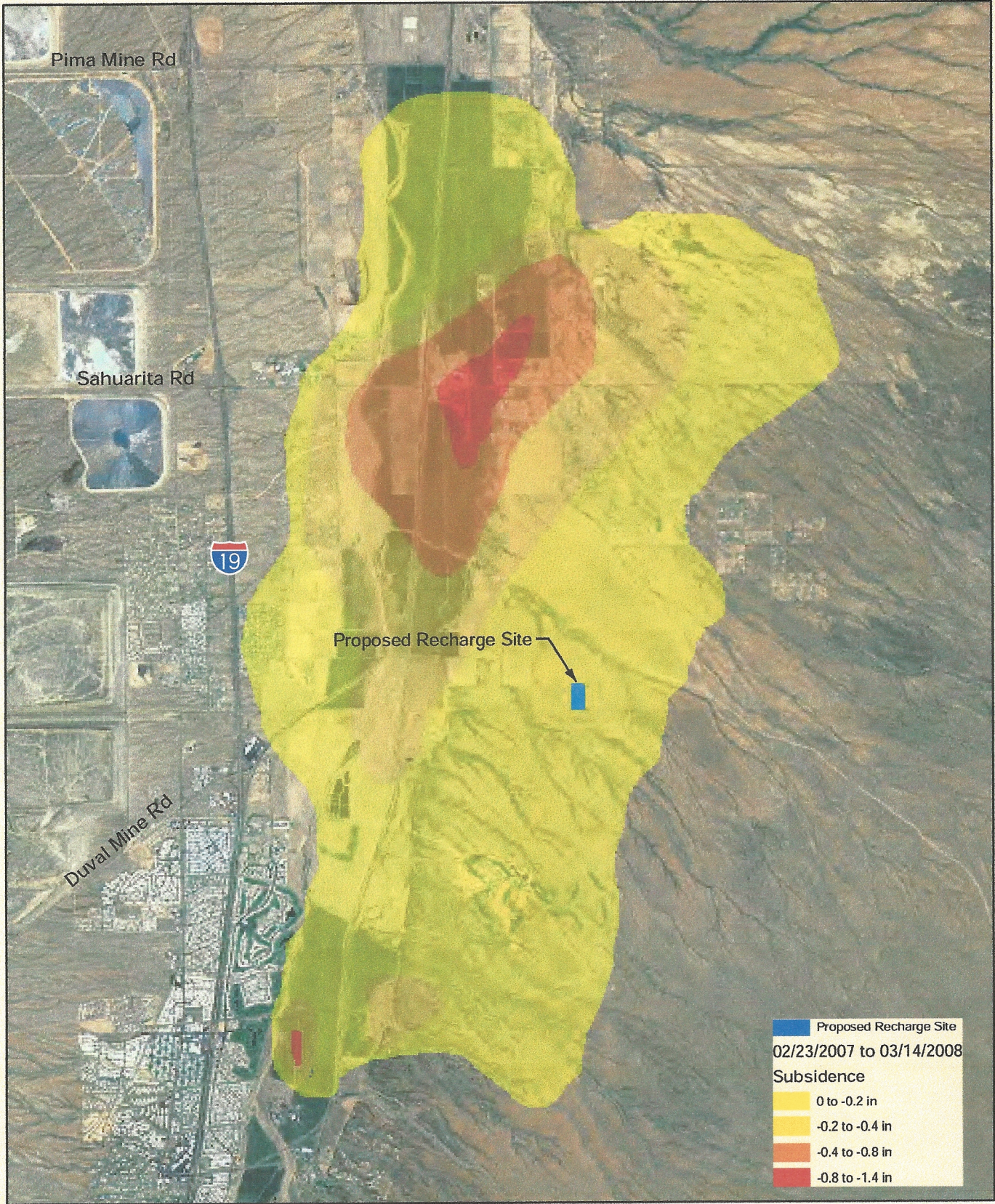
Figure 8 Regional Subsidence
